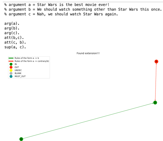
Figure 1: Example of our system deciding the winning arguments of a debate. The top picture shows the input file to our system, the bottom picture shows the calculated extension (under preferred semantics). In this case arguments a and c constitute the winning set of arguments.
